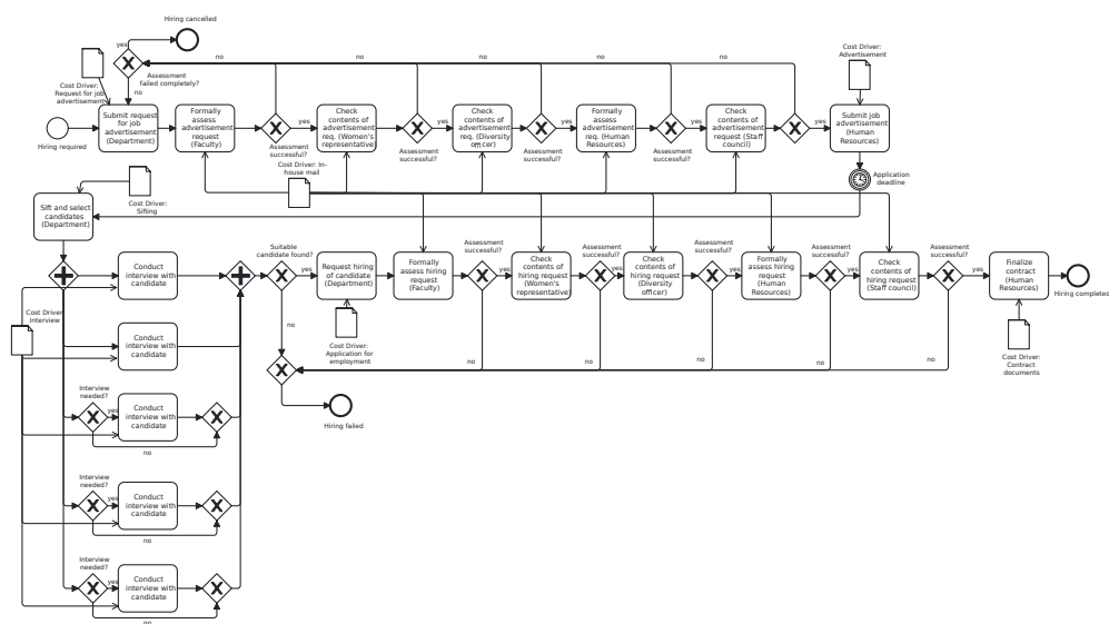
Fig. 13 BPMN diagram of the hiring process, with annotated abstract environmental cost driver
